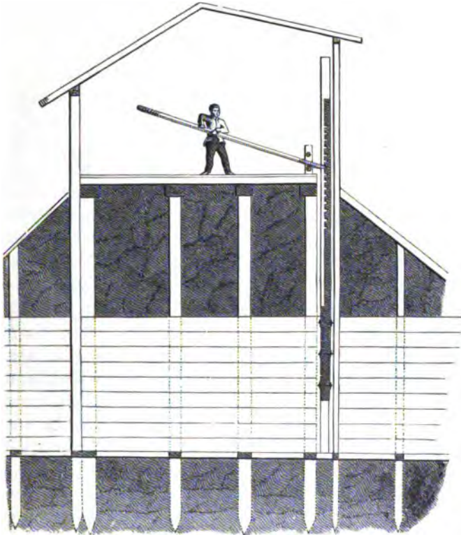
Fig. 238.—Earthen dam with sluice-valve.
